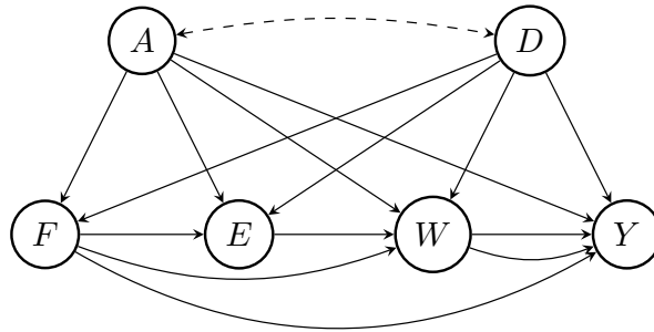
Figure 8: The causal graph for the government-census dataset. D are demographic features, A is gender, F represents marital and family information, E education, W work-related information and Y the salary, which is also the outcome of interest. The bidirected edge between A and D represents that the noise variables U_A and U_D share information.
